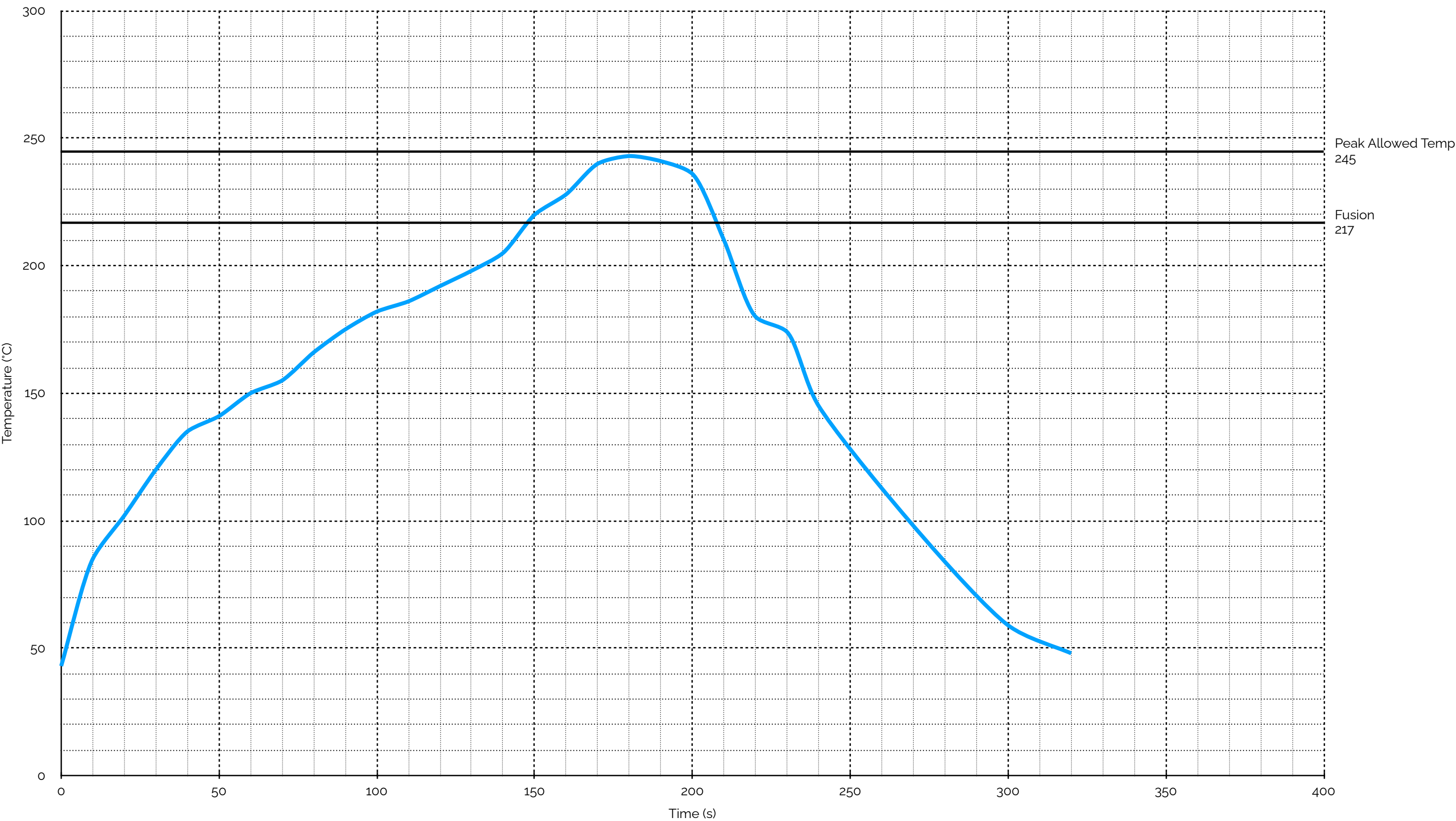
Typical Reflow Profile
